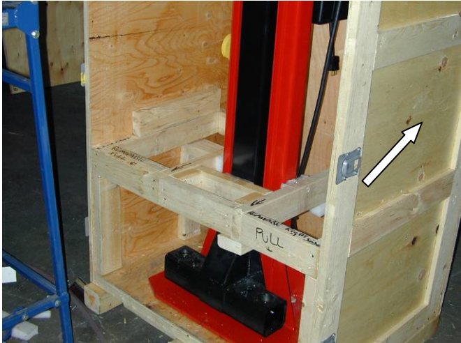
Figure 7 - Shipping crate Note the plywood identified by the arrow is exempt
